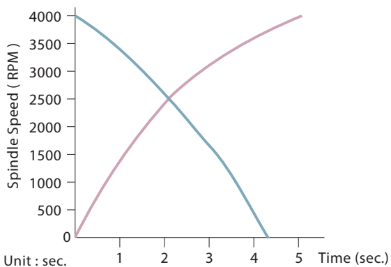
GA-2000 Spindle Acc. / Dec. Times Chuck : 10" + Hard Jaws
